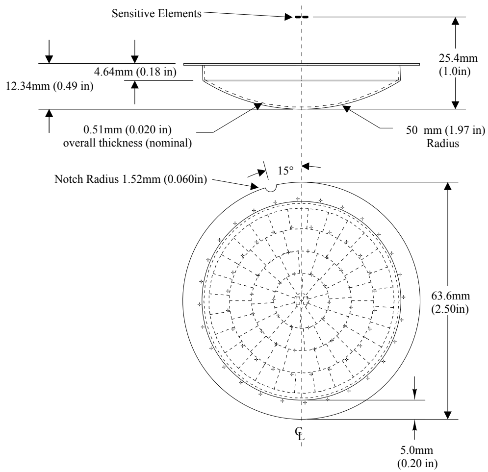
CM 1.0 GI VX-F MOUNTING GEOMETRY
