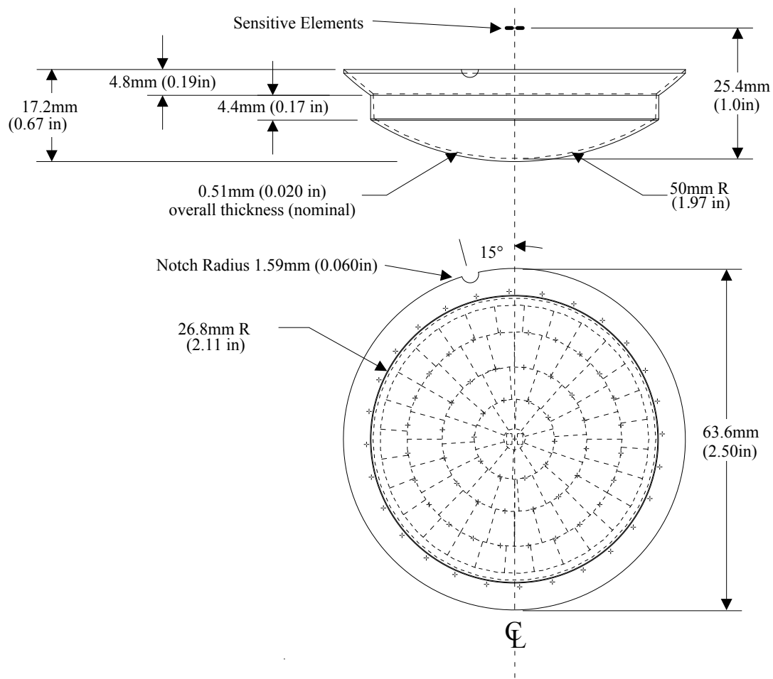
CM 1.0 GI VX MOUNTING GEOMETRY
